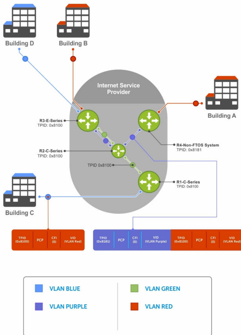
Figure 105. Single and Double-Tag TPID Match
